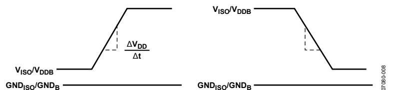
Figure 21. Transient Immunity Waveforms, Output Supplies
