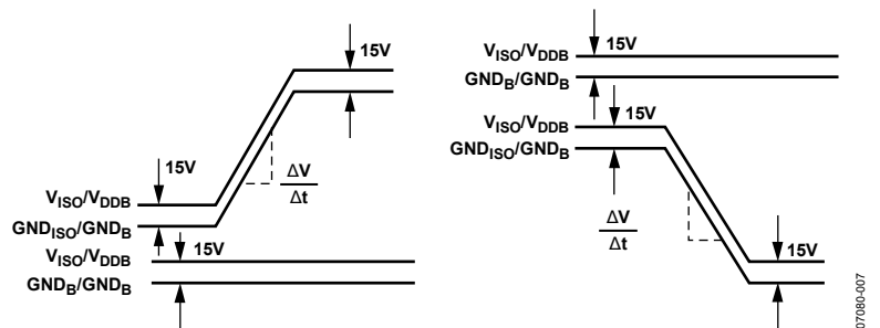
Figure 20. Common-Mode Transient Immunity Waveforms Between Outputs
