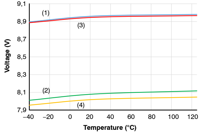
(1) V_{UVLOA-OUT-ON} (2) V_{UVLOA-OUT-OFF} (3) V_{UVLOB-OUT-ON} (4) V_{UVLOB-OUT-OFF}
