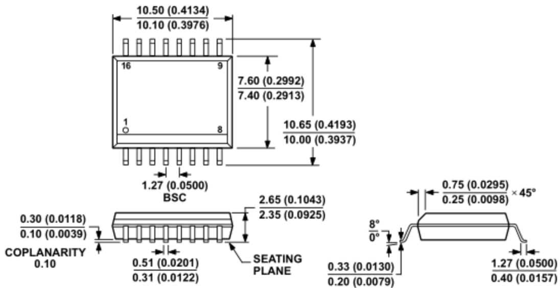
Figure 2. Wide Body SOIC-16 Packaging
