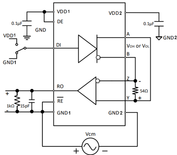
Figure 9. Common-Mode Transient Immunity Test Circuit
