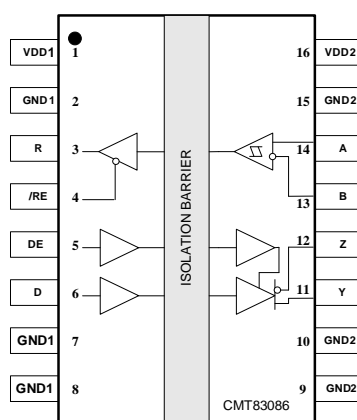
Figure 1. CMT83086 Pin List
